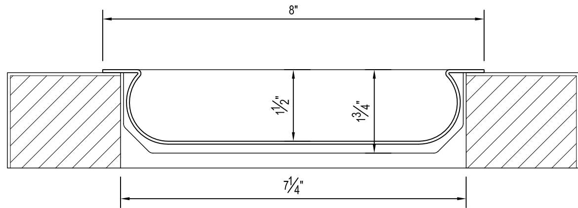
1 SECTION
